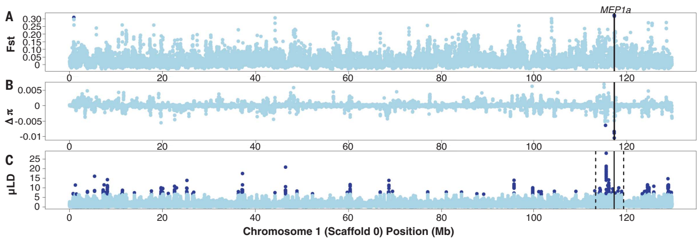
Fig. 3. Autosomal candidate locus for tusklessness in Gorongosa elephants.
